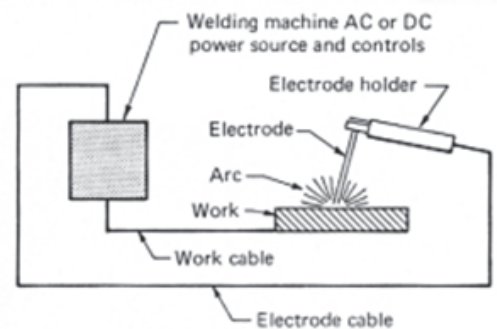
Fig. 1. The basic arc-welding circuit
