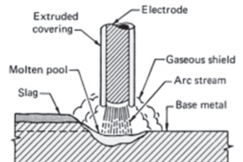
Fig. 2 This shows how the coating on a coated (stick) electrode provides a gaseous shield around the arc and a slag covering on the hot weld deposit.
